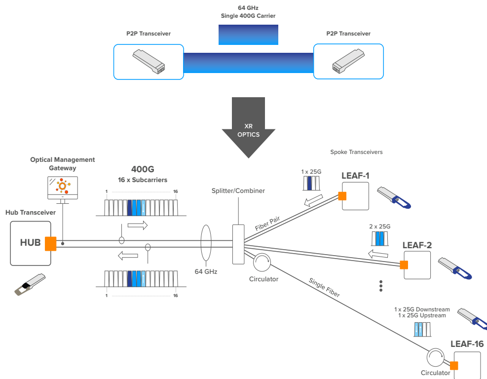
Figure 1: Point-to-multipoint coherent with 25 Gb/s digital subcarriers
