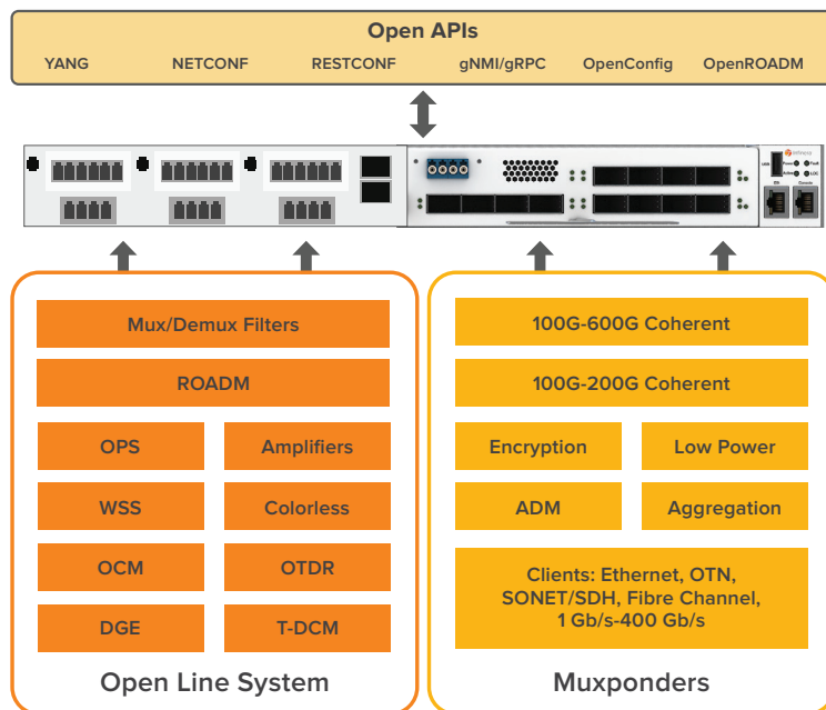
Figure 1: The GX G30 Series: muxponder and metro OLS
