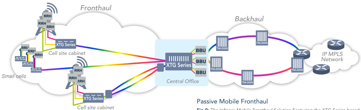
Fig 9: The Infinera Mobile Fronthaul Solution Featuring the XTG Series-based Passive WDM Option Enabling Low – or Even No – Power Consumption.
