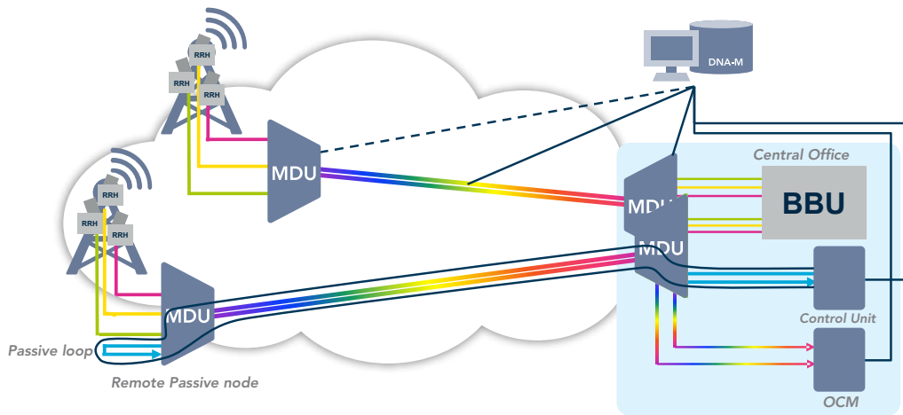
Fig 7: The Infinera Semi-passive Mobile Fronthaul Provides Passive Wavelength Monitoring Capabilities to Allow More Advanced OAM. Only Macro Cell Deployments Are Shown in this Example, but the Semi-passive Option Is Equally Beneficial in Small Cell Deployments.
