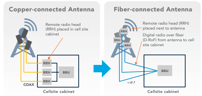
Fig 1: Fiber-connected Antennas Allow the RRH to Be Placed with the Antenna, Bringing Advantages Such as Lower Power Consumption at Cell Sites, Whether They Are Small Cells or Macro Cells
