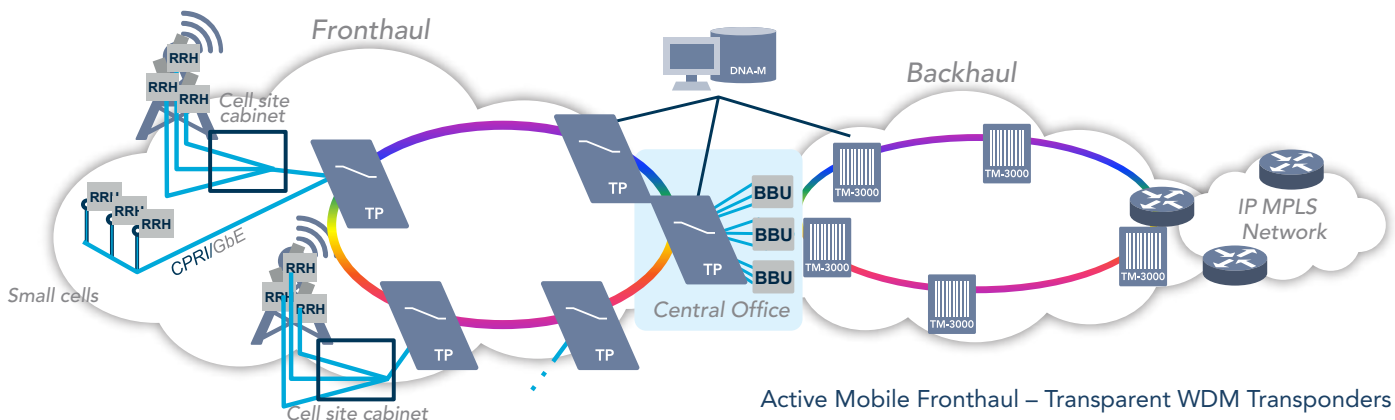
Fig 6: The Infinera Active Mobile Fronthaul Uses the Active XTM Series Transparent Transponders, Bringing Key Values such as Low Latency and Superior Sync.
