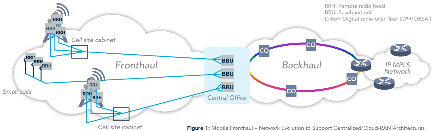
Figure 1: Mobile Fronthaul – Network Evolution to Support Centralized/Cloud-RAN Architectures
